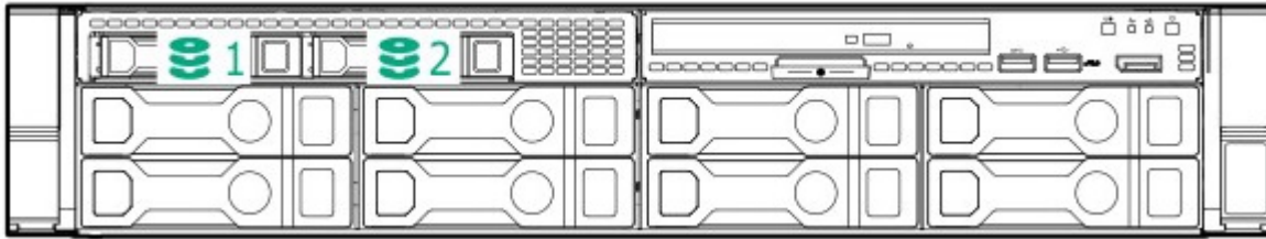
8LFF chassis with Universal media bay and optional 2SFF and optical drive shown
